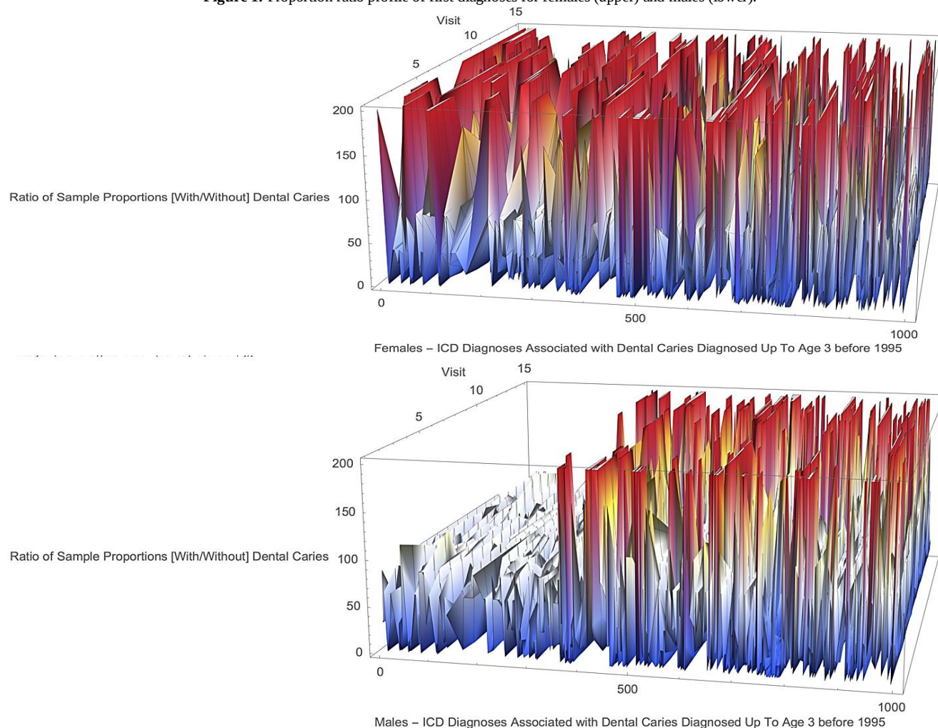
Figure 2: Proportion ratio profile of first 15 diagnoses for females (upper) and males (lower).
