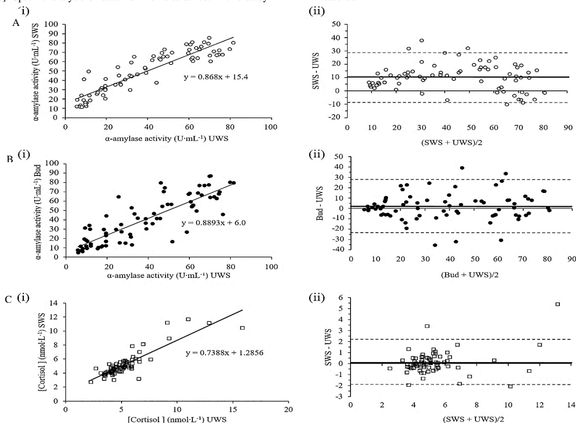
Figure 3: Association and agreement between A ) SWS and UWS for \alpha -amylase activity ( r=0.908 ); B ) Bud and UWS for \alpha -amylase activity ( r=0.851 ); and C ) SWS and UWS for cortisol levels ( r=0.868 ). The linear relationship and its equation for each pair is shown in i ), with the associated Bland-Altman absolute difference plots alongside ii ) Bland-Altman plots show the mean difference ( \bar{d} ) as a thick solid black line and the corresponding positive and negative limits of agreement as hashed lines. Values for each parameter are above or below each line.
