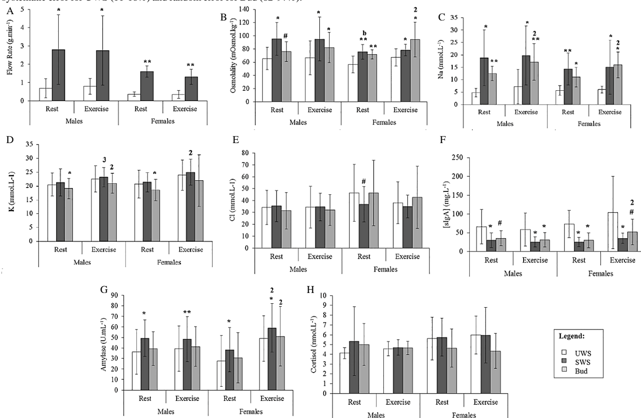
Figure 2: Comparison between the means of each method for A) flow rate ( \text{g}\cdot\text{min}^{-1} ); B) osmolality ( \text{mOsmol}\cdot\text{kg}^{-1} ); C) Na ( \text{mmol}\cdot\text{L}^{-1} ); D) K ( \text{mmol}\cdot\text{L}^{-1} ); E) Cl ( \text{mmol}\cdot\text{L}^{-1} ); F) slgA ( \text{mg}\cdot\text{L}^{-1} ); G) \alpha -amylase activity ( \text{U}\cdot\text{mL}^{-1} ); and H) cortisol ( \text{nmol}\cdot\text{L}^{-1} ), for males and females during both rest and exercise. A significant difference between SWS/Bud and UWS is indicated with an asterisk (**, P<0.001 ; *, P<0.05 ) and a trend for this difference with a superscript hash (#, 0.1<P>0.05 ). For comparisons between rest and exercise within a method, significance is shown on the latter variable by number (1, P<0.001 ; 2, P<0.05 ; 3, 0.1<P>0.05 ). For comparisons between males and females within a method, significance is shown on the latter variable by letter (a, P<0.001 ; b, P<0.05 ).
