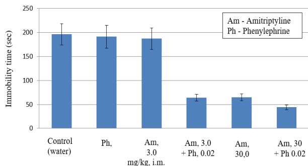
Figure 1: Antidepressant effect of amiripryline, phenylephrine and their combinations in the Porsolt test (in rats). The anti-depression effect of drugs on the durations of immobility in the forced swim test. During the 5 min test, the duration of immobility was observed and measured.
