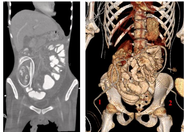
Figure 2: CT abdomen/pelvis (coronal view) with 80 cc of Omnipaque 350 intravenous contrast using 3 mm increments obtained. Figure on left illustrates the location of intraabdominal drains following closure. Figure on right is a multiplanar volume rendering technique demonstrating intraabdominal drain placement in relation to the bowel. Label 1 was the drain that instilled the DPR solution. Label 2 is an additional drain that was inserted to monitor effluent surrounding bowel perforation.
